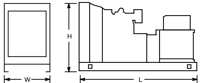
NOTE: This drawing is provided for reference only and should not be used for planning installation. Contact your local distributor for more detailed information.
